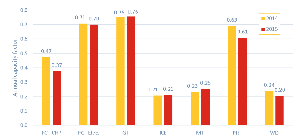
Figure 5-31: 2014 and 2015 Annual Capacity Factors by Technology
