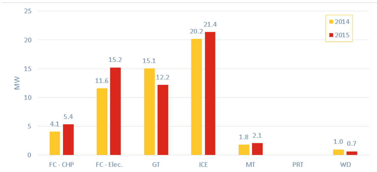
Figure 5-18: SCE 2014 & 2015 Peak Hour Generation by Technology
