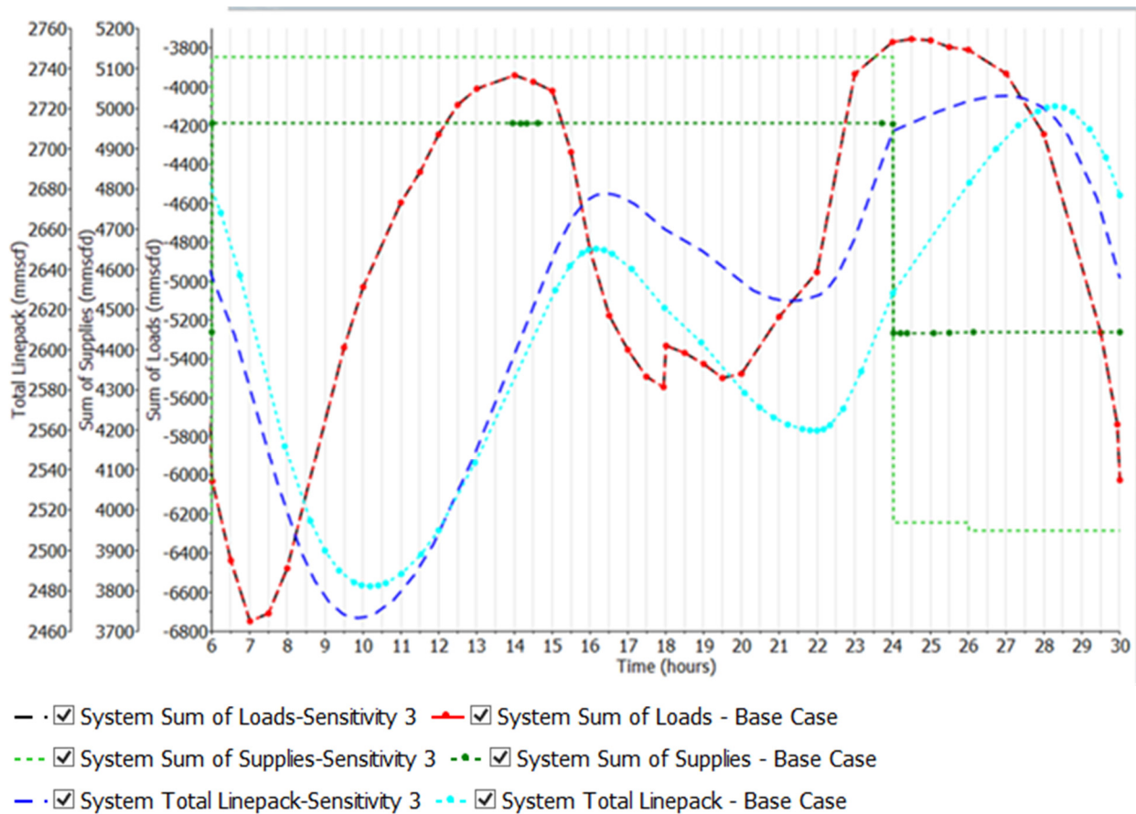
Figure III - 11 Sensitivity 3 – Non-Aliso Inventory 37% Loads, Supplies, Linepack - Overlaid with Base Case
