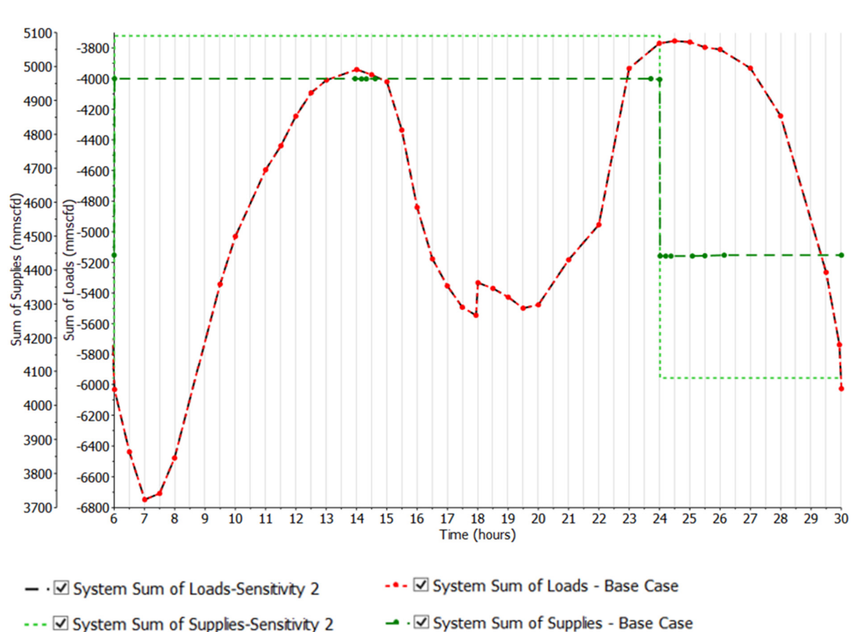
Figure III - 8 Sensitivity 2 – Non-Aliso Inventory 50% Loads and Supplies - Overlaid with Base Case
