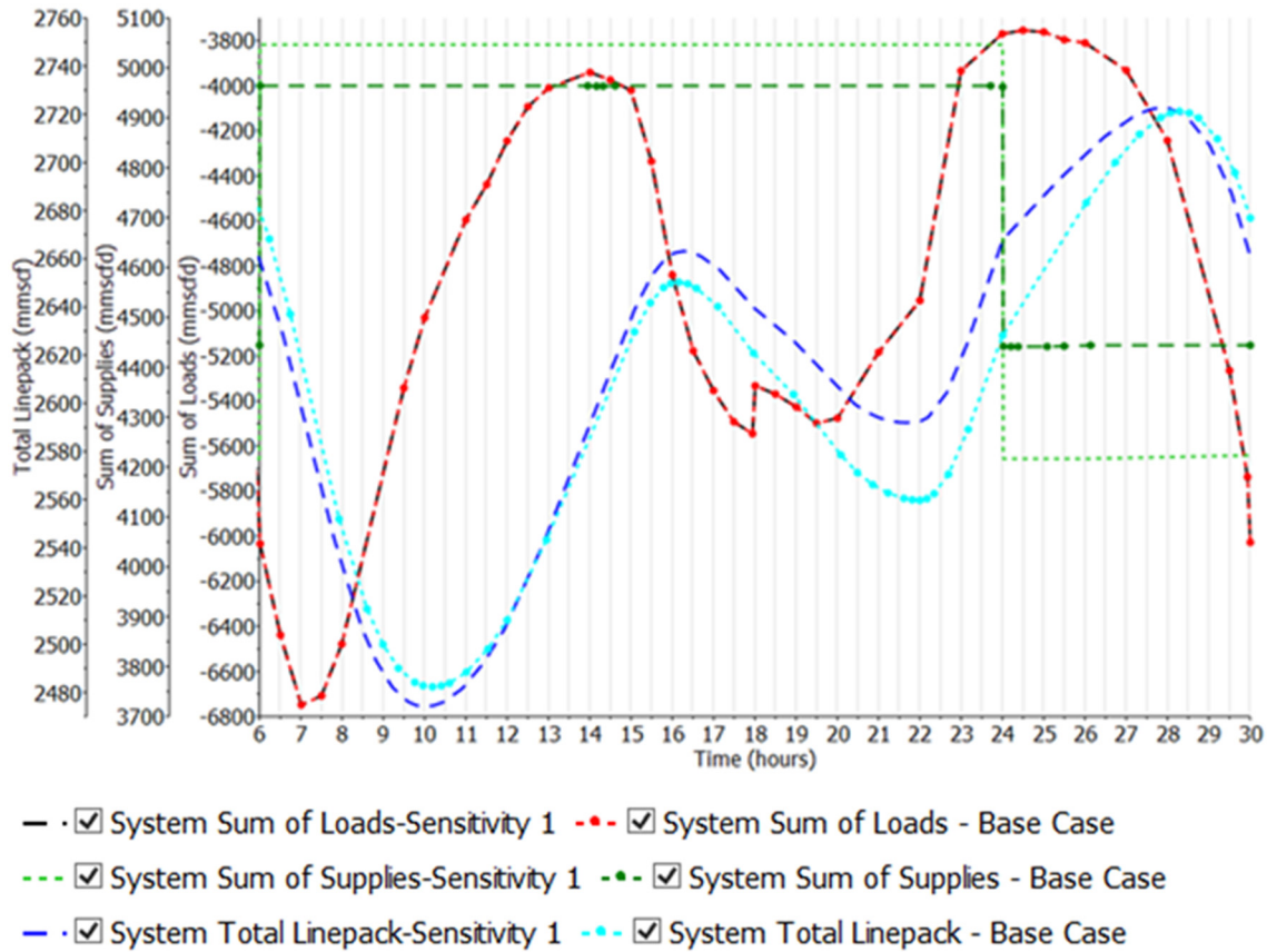
Figure III - 6 Sensitivity 1 – Non-Aliso Inventory 70% Loads, Supplies and Linepack — Overlaid with Base Case
