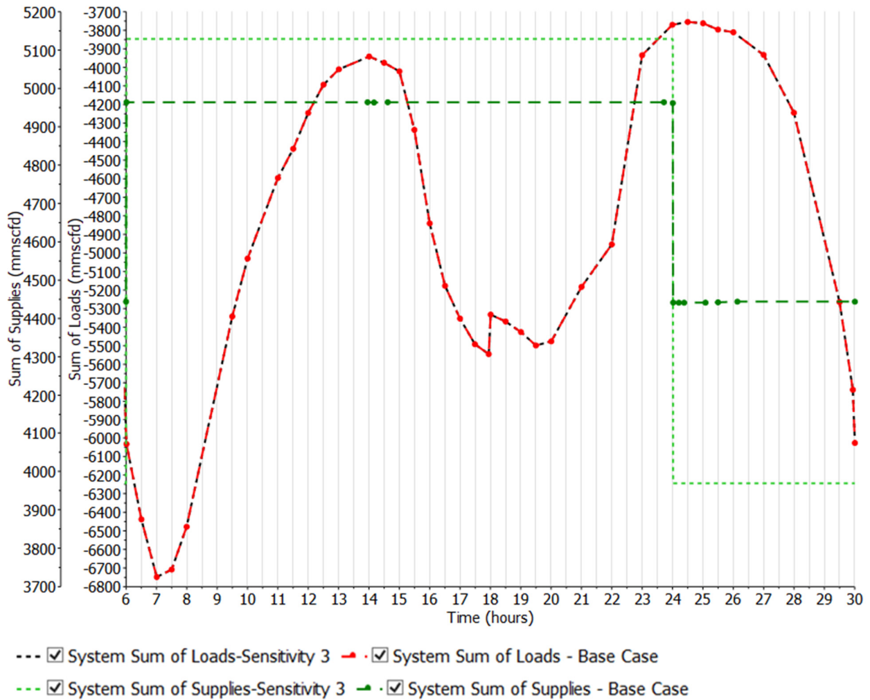
Figure III - 10 Sensitivity 3 – Non-Aliso Inventory 37% Loads and Supplies - Overlaid with Base Case
