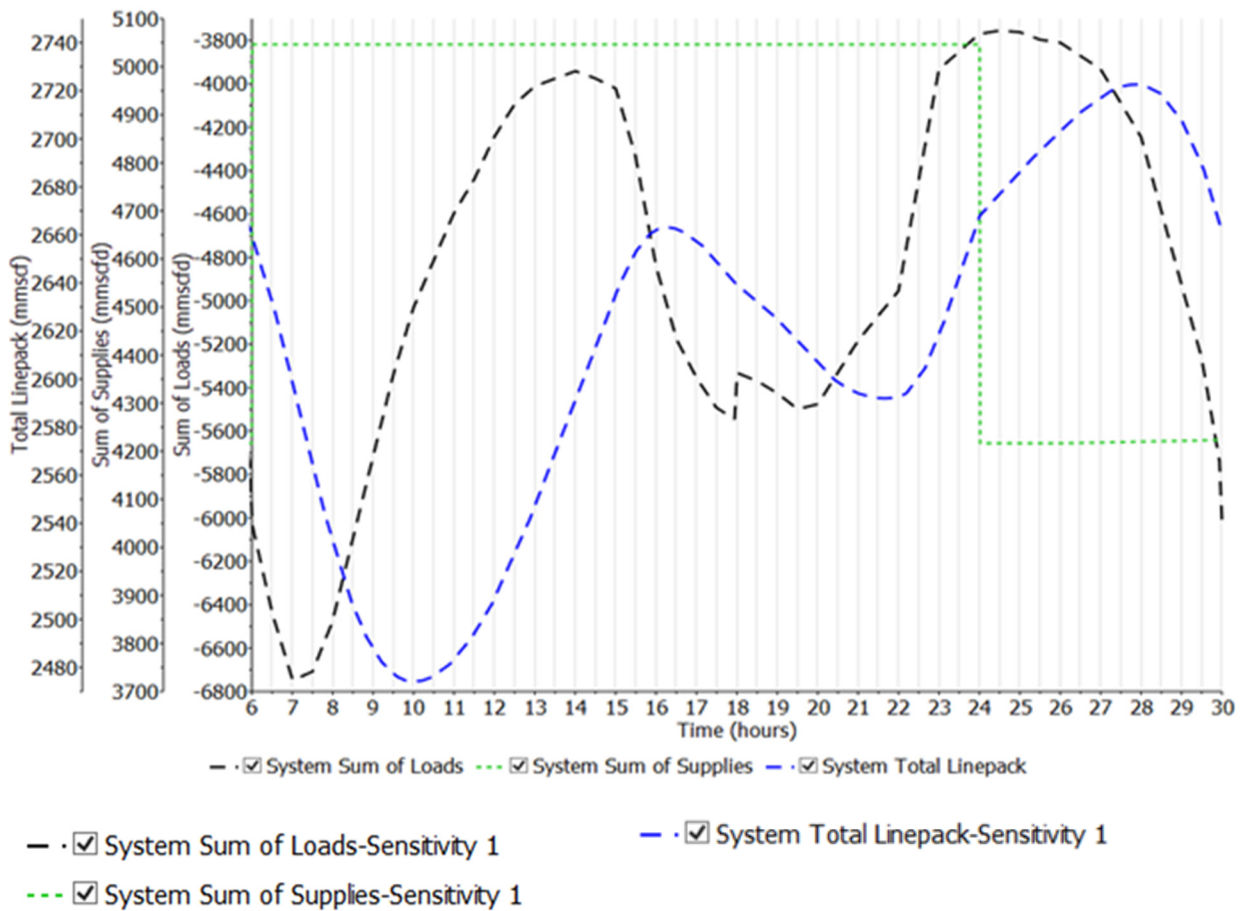
Figure III - 4 Sensitivity 1 – Non-Aliso Inventory 70%: Loads, Supplies and Linepack
