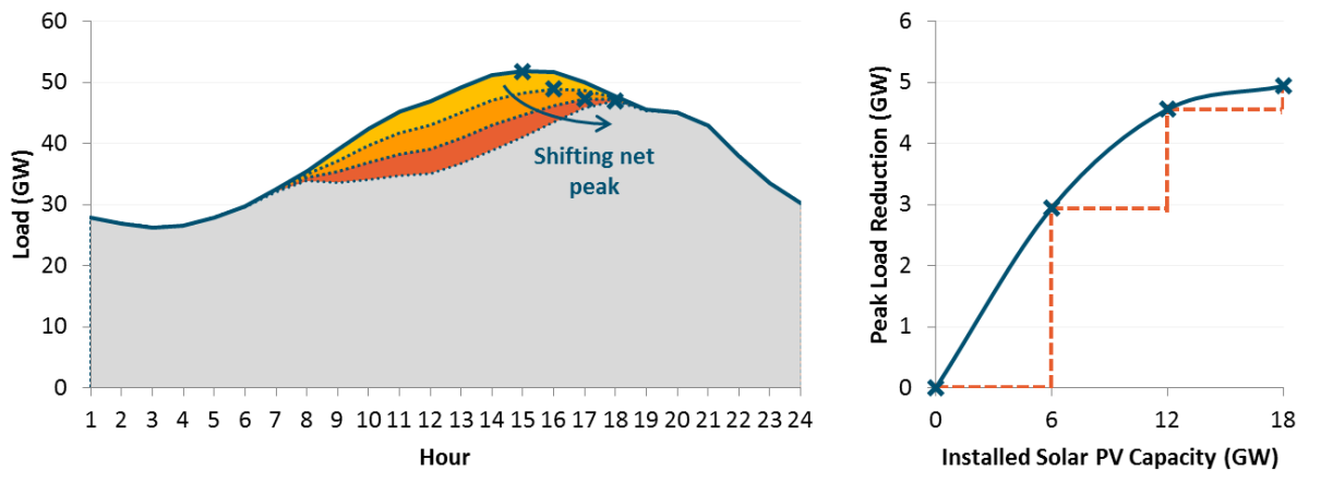
Figure 7.1. Illustrative example of the declining marginal ELCC of solar PV with increasing penetration 48
