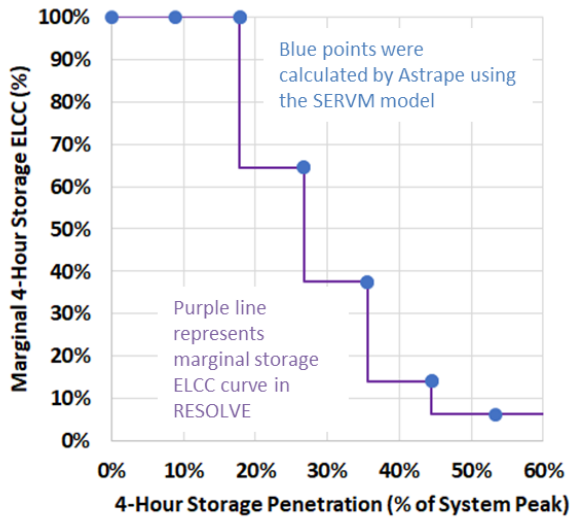
Figure 7.2. Battery Storage ELCC Curve
