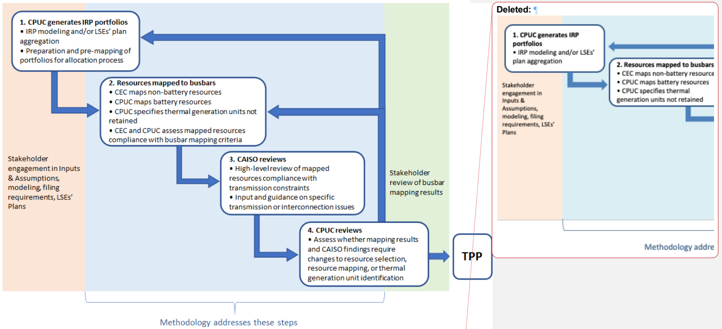
Figure 1. Flowchart of the busbar mapping process
